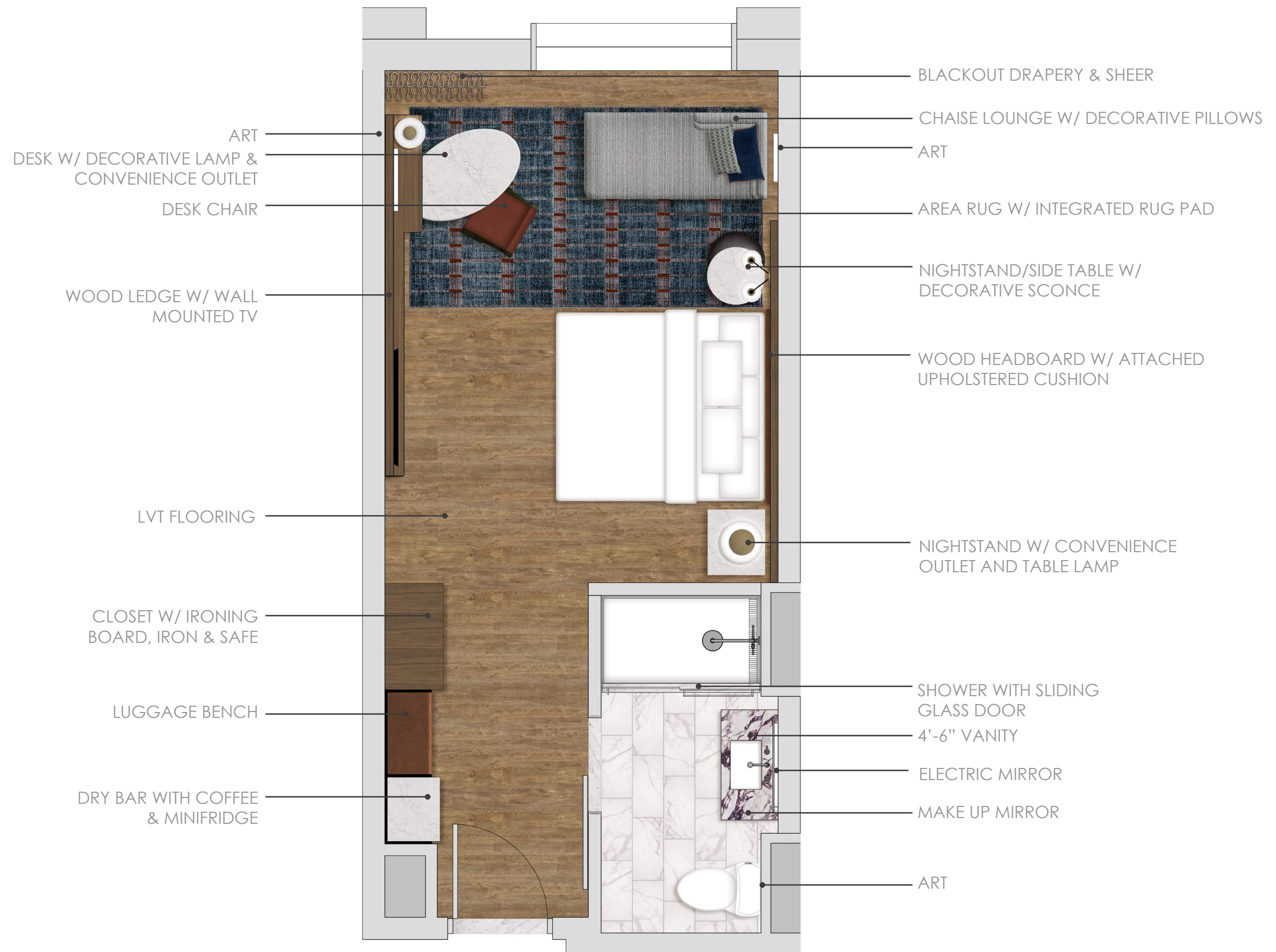
KING GUESTROOM FLOOR PLAN ID SCHEMATIC DESIGN PRESENTATION | 09.17.25
