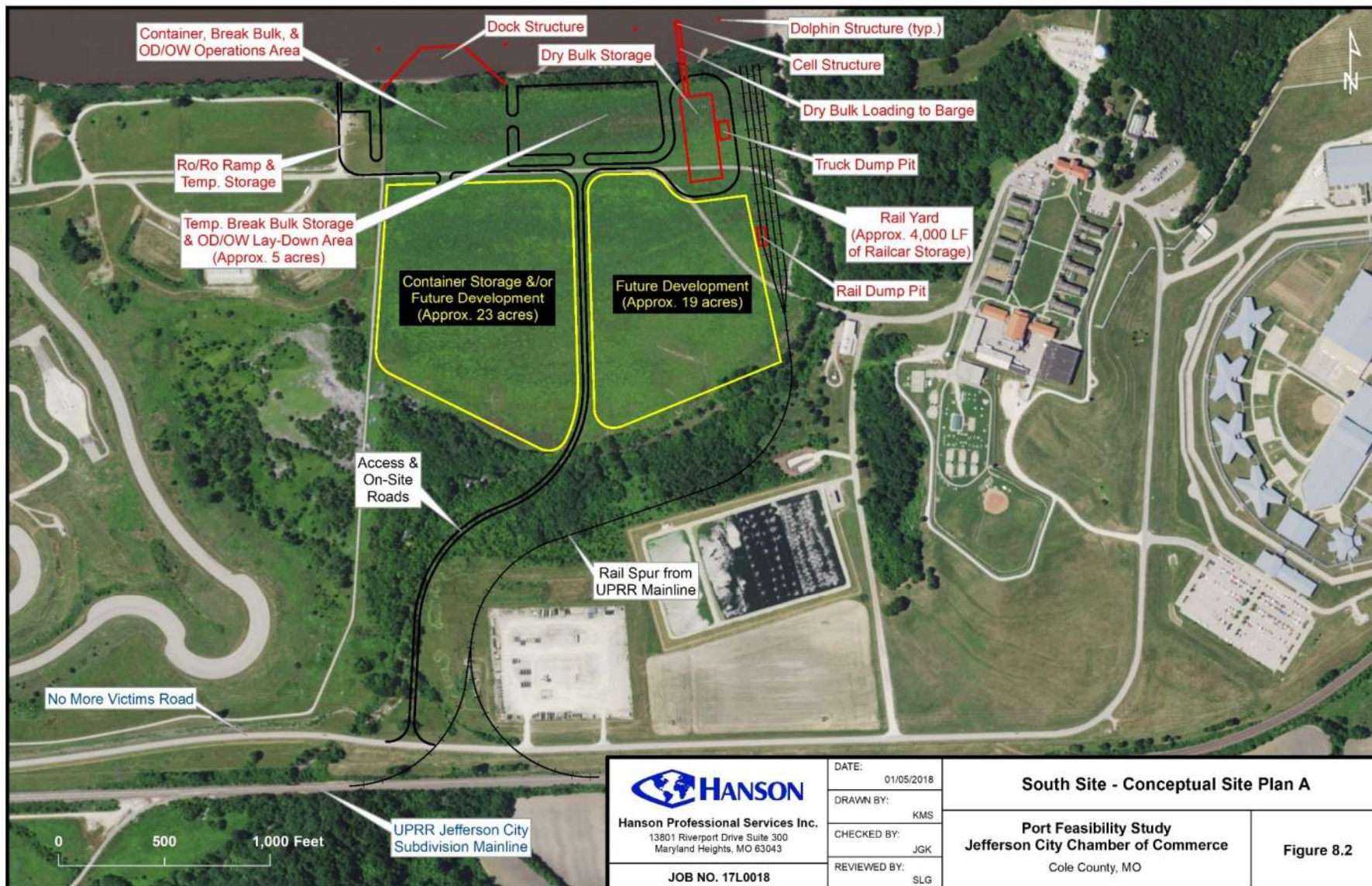
Figure 8.2 South Site – Conceptual Site Plan A
